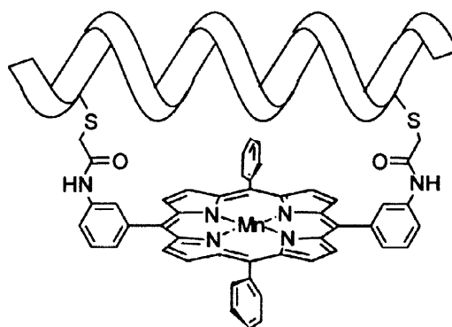
Figure 1. Mn(III)porphyrin-peptide conjugate.
